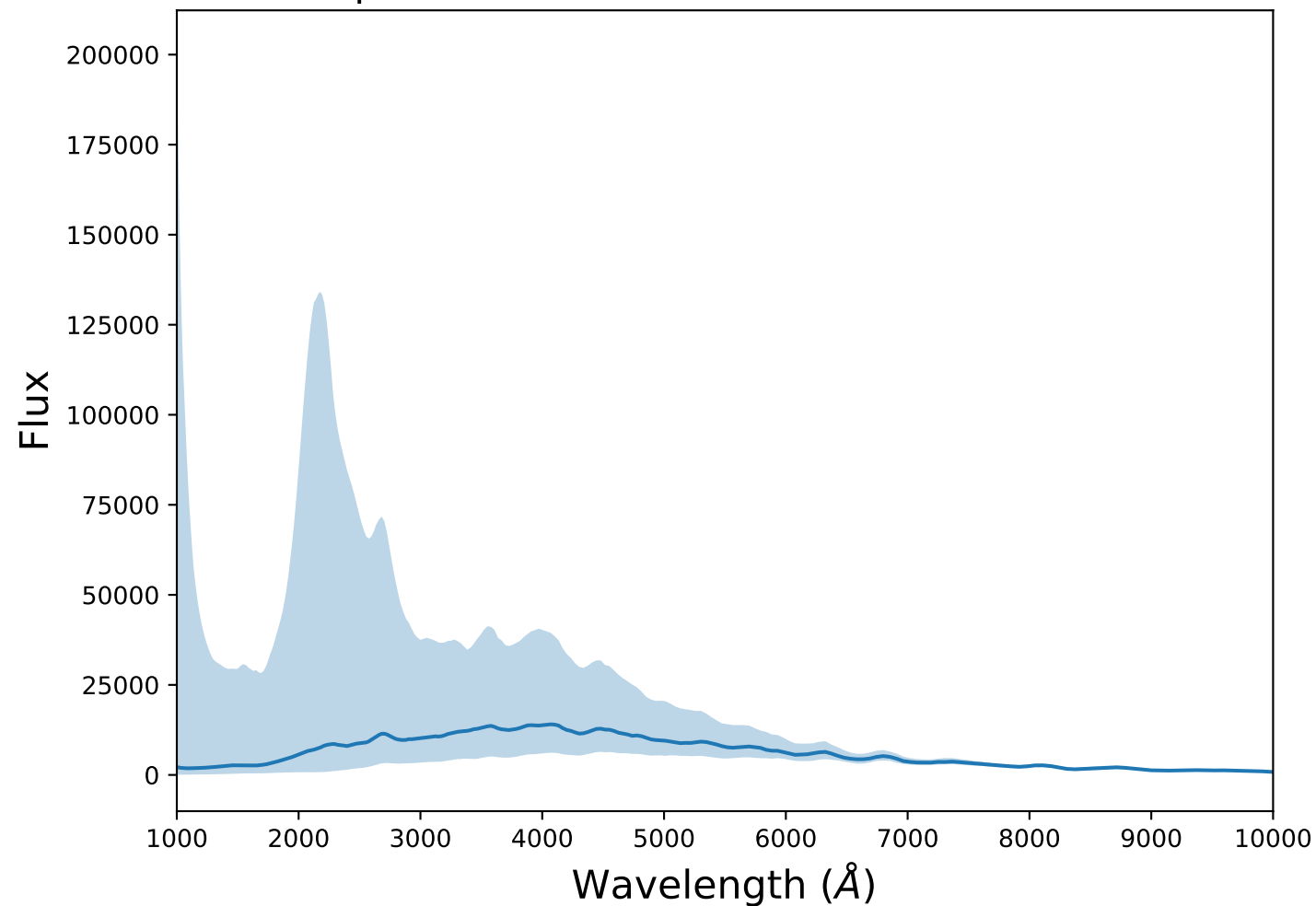
Spectrum 2 for transient SNIa at z=0.27
